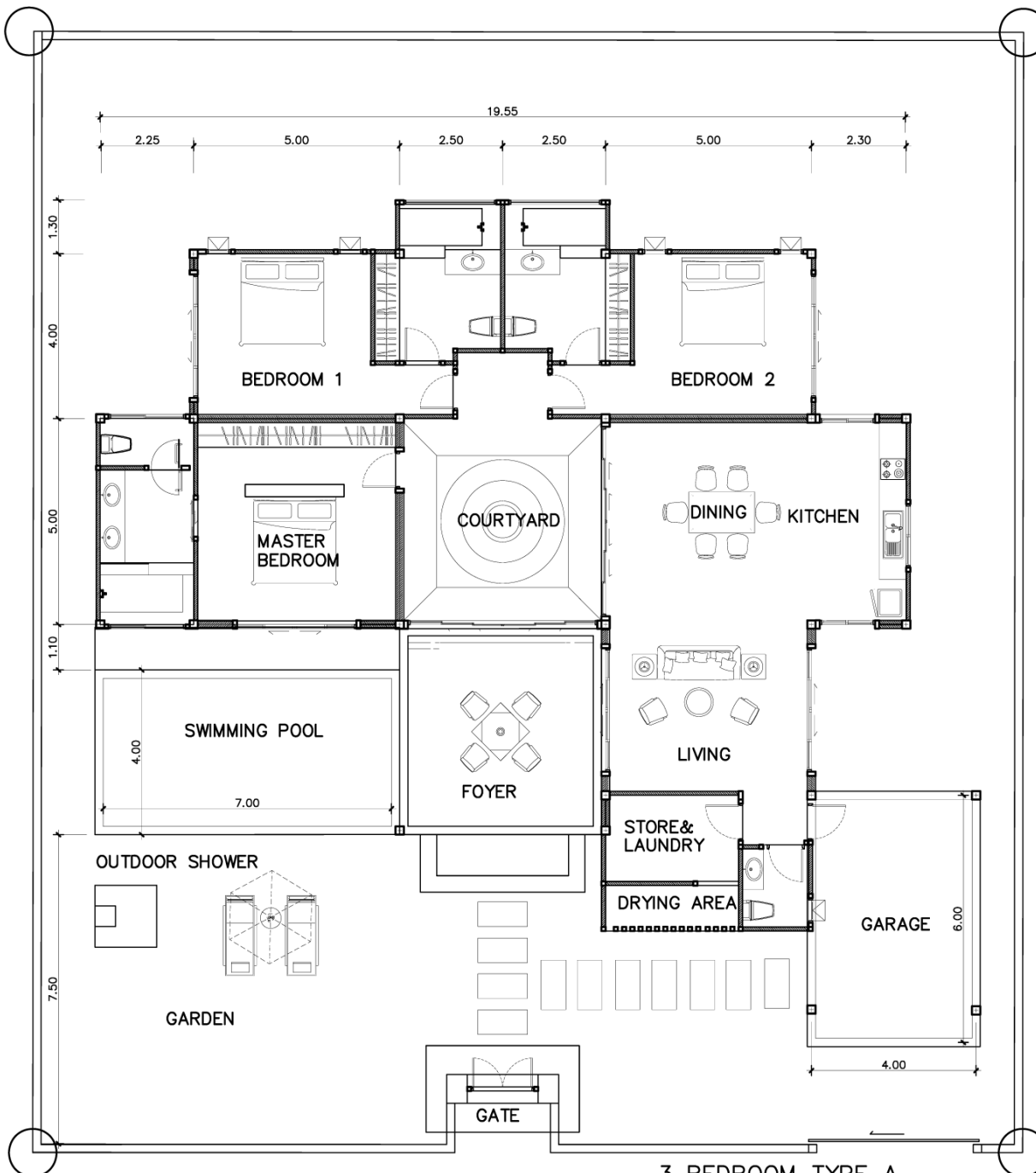
3 BEDROOM TYPE A GROUND FLOOR PLAN
